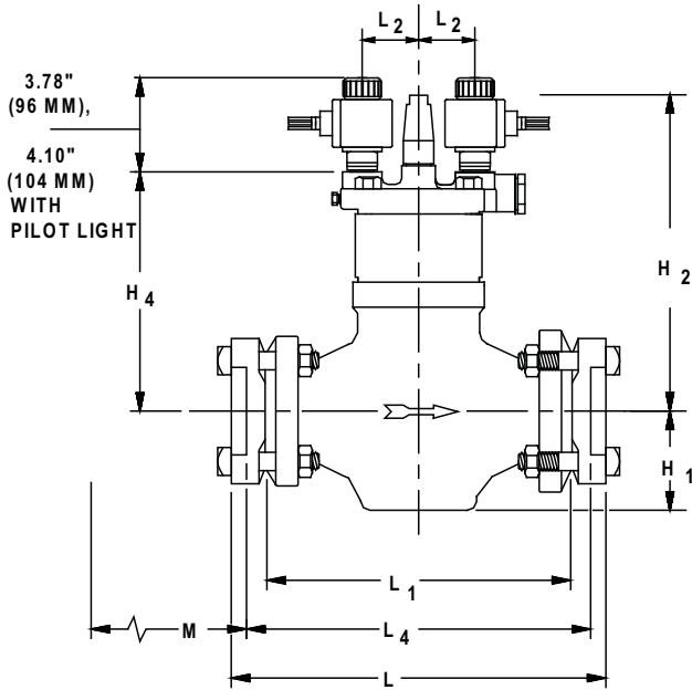
HS4D FLANGED VALVE
