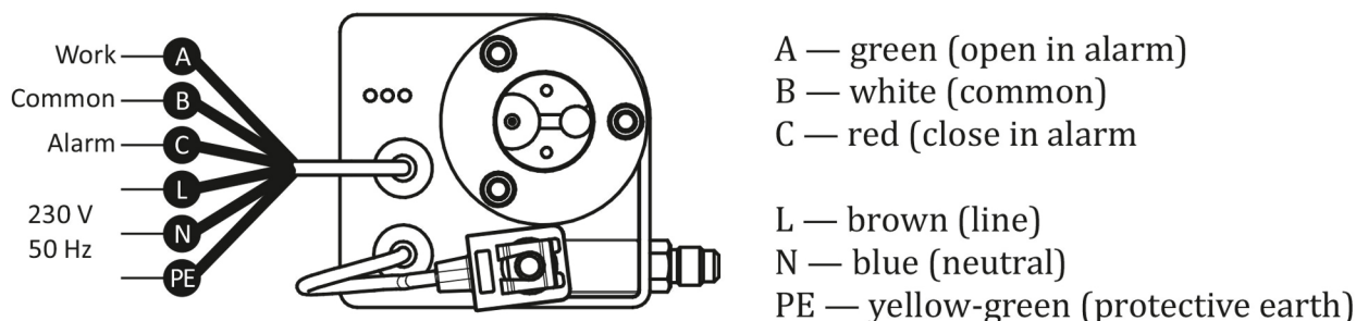
Fig.3. Electrical Connection
