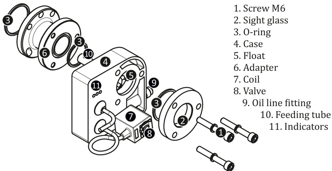
Fig.2. Assembly drawing
