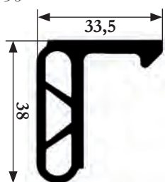
Bourrelet 8550 Gasket 8550
