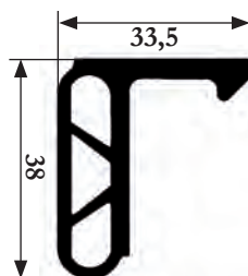
Bourrelet 8550 Gasket 8550
