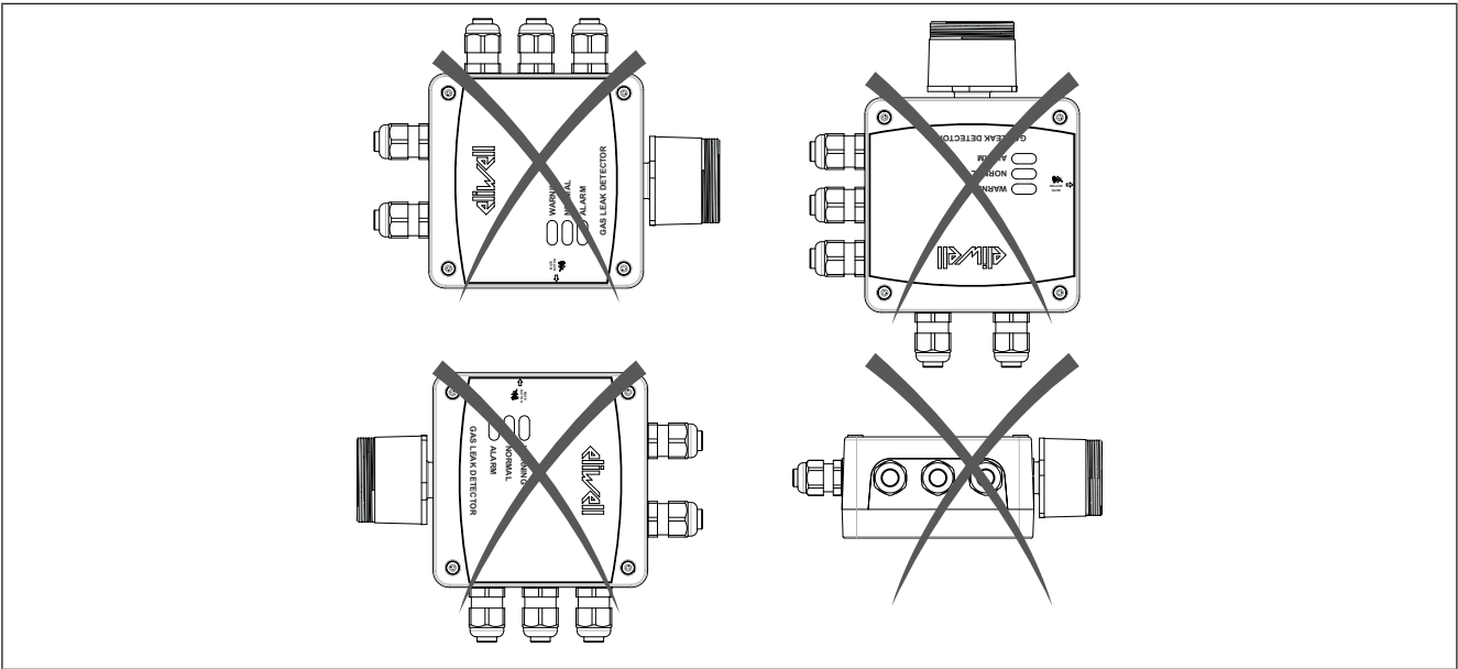
Fig. 10. Incorrect Mounting Position
