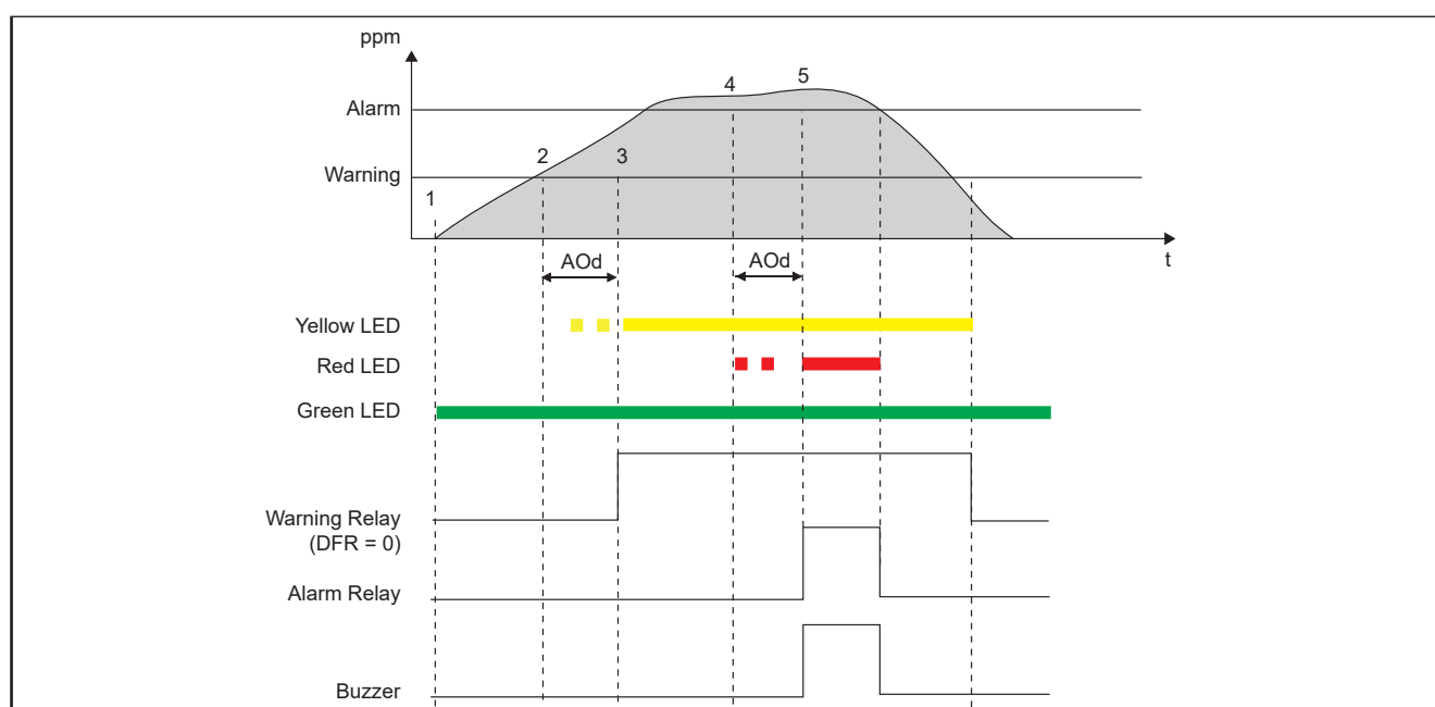
Fig. 22. Alarm/Warning sequences
