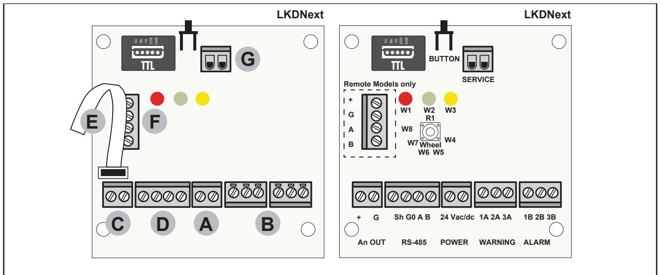
Fig. 13. Electrical connections
