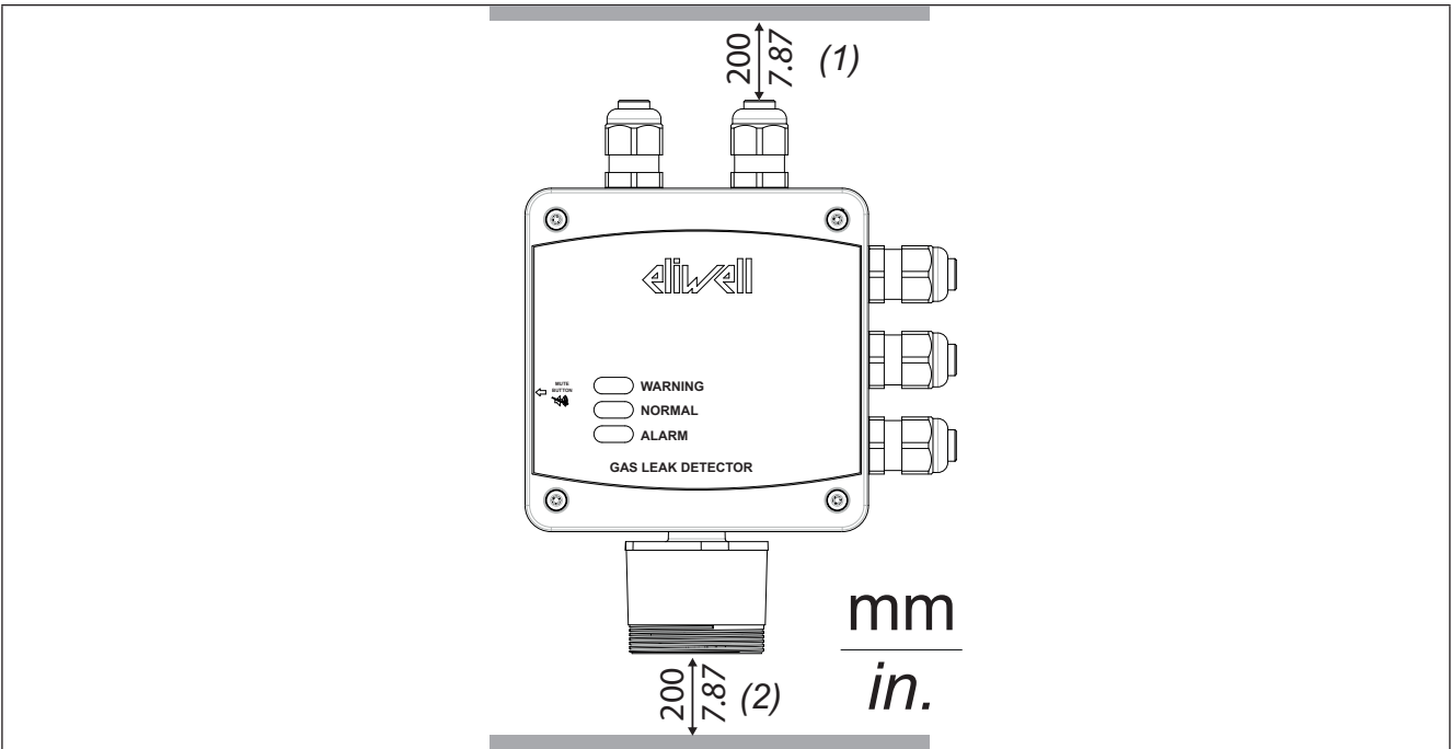
Fig. 11. Minimum Clearances
