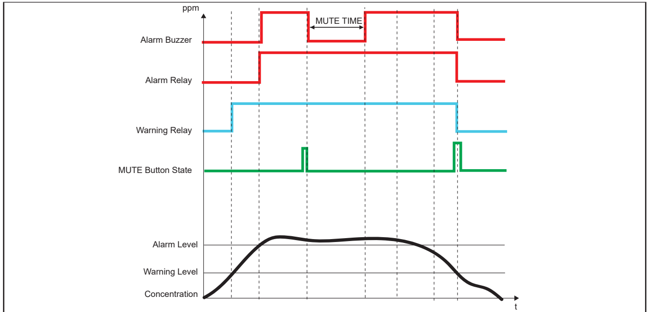
Fig. 24. Alarm/Warning sequences
