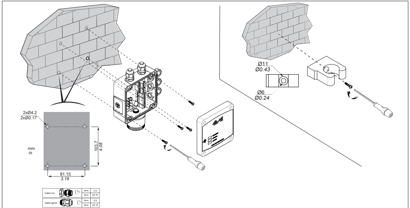
Fig. 1. LKDNext Mounting
