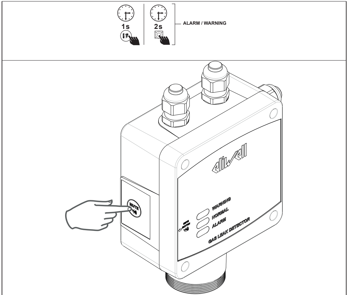
Fig. 25. Alarm / Acknowledge
